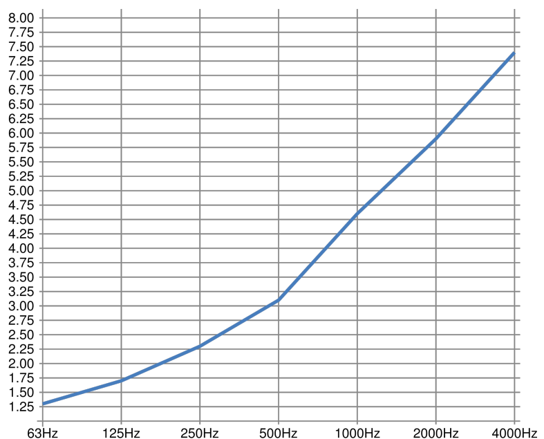
Equivalent sound absorption area / unit
